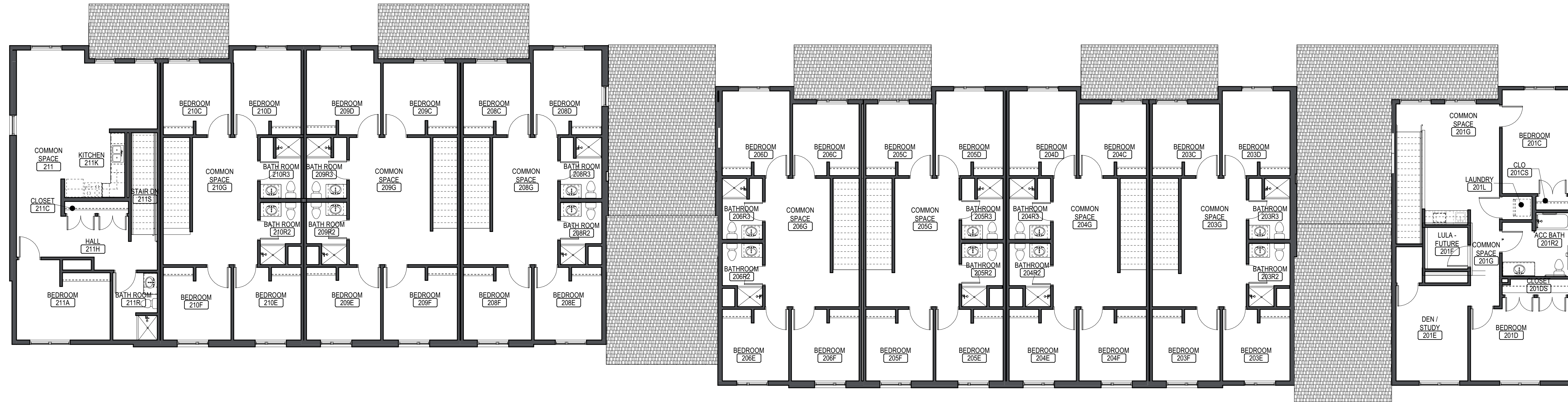
2 FLOOR PLAN - SECOND LEVEL ZONE 2 1/8" = 1'-0"
